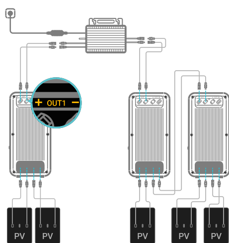
Diagram for Connecting 3 B2500-D
